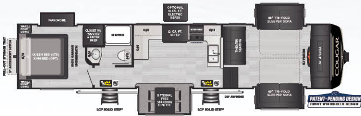
354FLS | Front living, pull-out rear storage tray WEIGHT 10910 LENGTH 39' 4"
