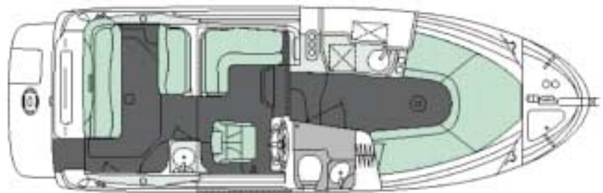
Floor Plan
