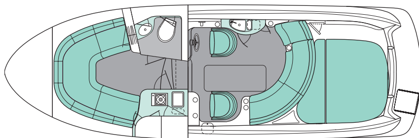
Cabin/Cockpit Layout w/Standard Seating
