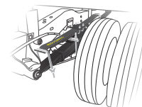
HELLWIG® HELPER SPRINGS Work with the chassis' existing springs to give the RV more support, improving stability under heavy loads
