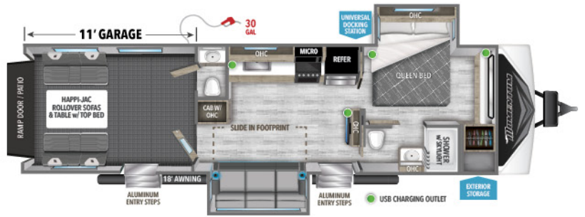
29G 11' GARAGE UVW' EMPTY HITCH' GVWR LENGTH' HEIGHT CAPACITY 8,700 1,500 13,000 33' 11" 12' 4" 96 37 39 37* * 1/2 BATH DOUBLES AS BLACK/GREY
