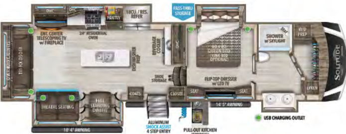
372WB UVW' HITCH' GVWR LENGTH' HEIGHT CAPACITY 372WB-R 13,950 2,800 16,800 41' 4" 13' 5" 93 100 50
