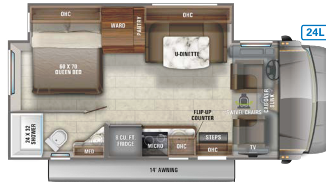
Ext. Lgth: 25' 2" Wheelbase: 170" GVWR: 11,030 lbs.
