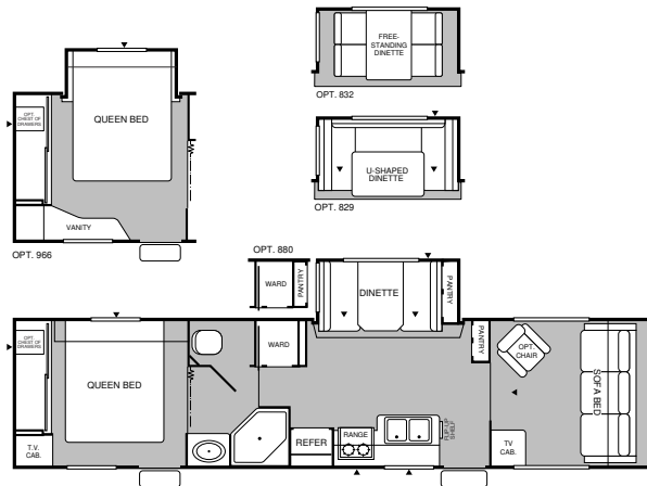
31 5R fifth wheel
