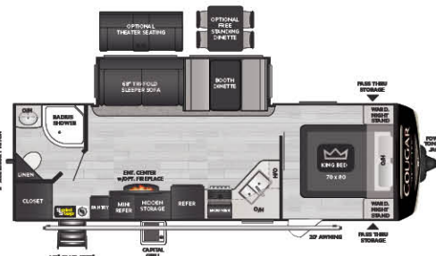
26RBSWE Rear bath w/ outside kitchen WEIGHT 6646 LENGTH 29' 11"
